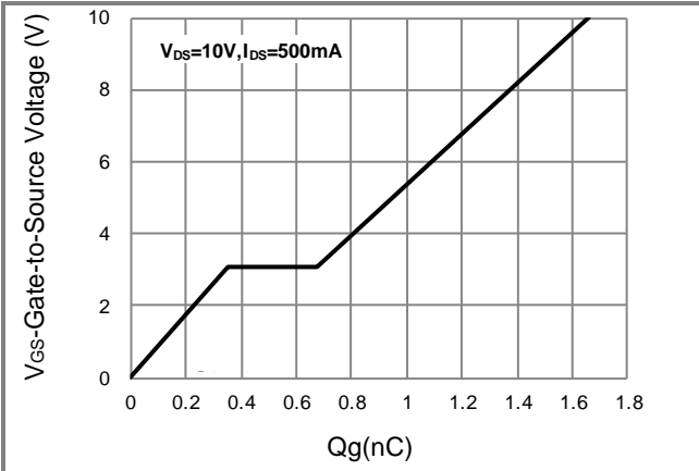
Fig.7 Gate-Charge Characteristics
