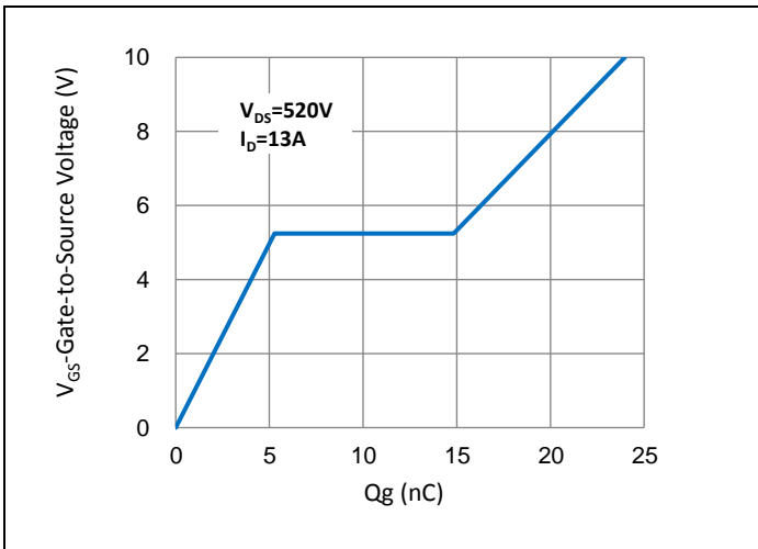
Fig.7 Gate-Charge Characteristics
