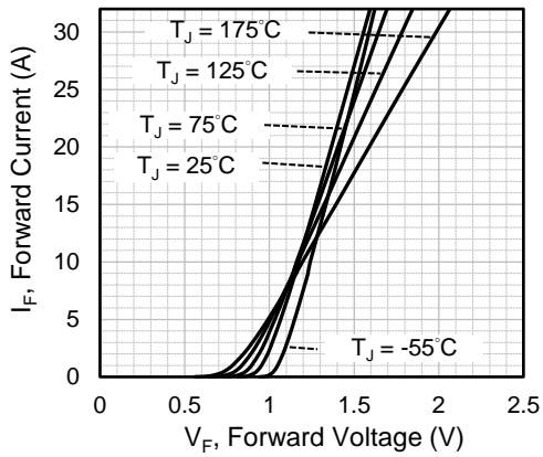
Fig.1 Forward Characteristics
