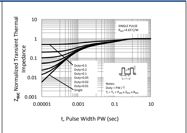
Fig.12 Normalized Transient Thermal Impedance
