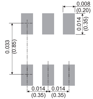
DFN2020-6L
