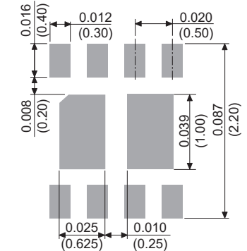
DFN2020-8L
