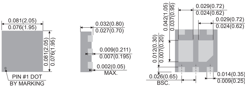
DFN2020-6L
