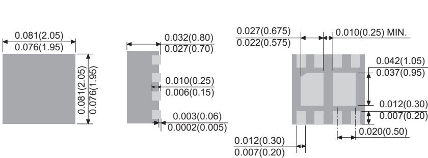
DFN2020-8L
