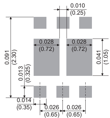
DFN2020-6L
