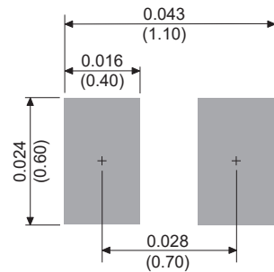
DFN1006-2L
