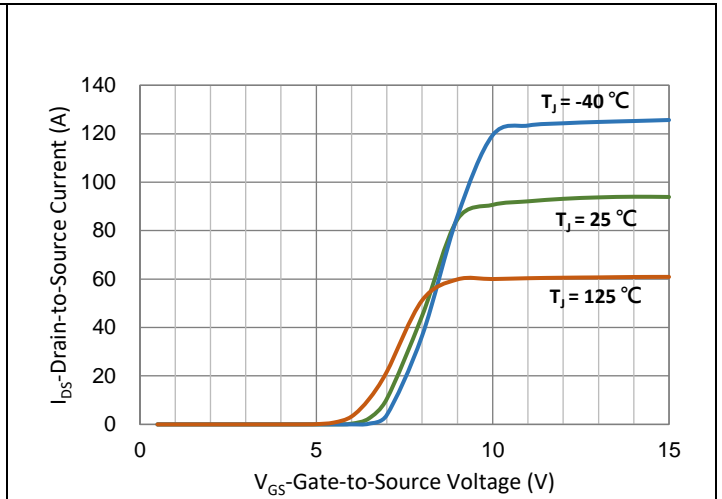
Fig.2 Transfer Characteristics
