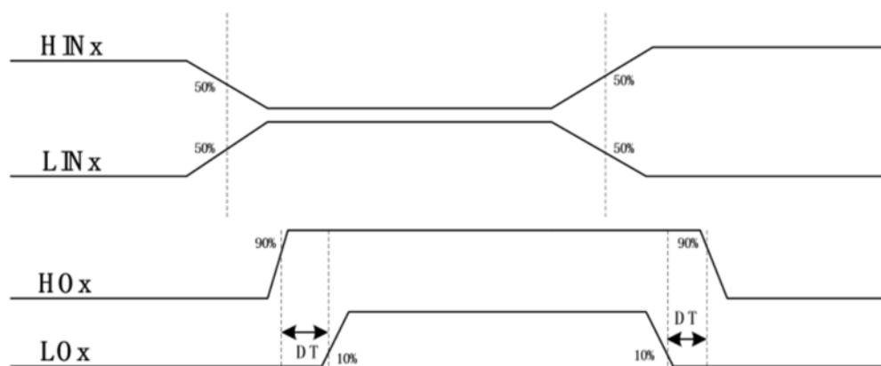
Figure 3-7 Dead Time
