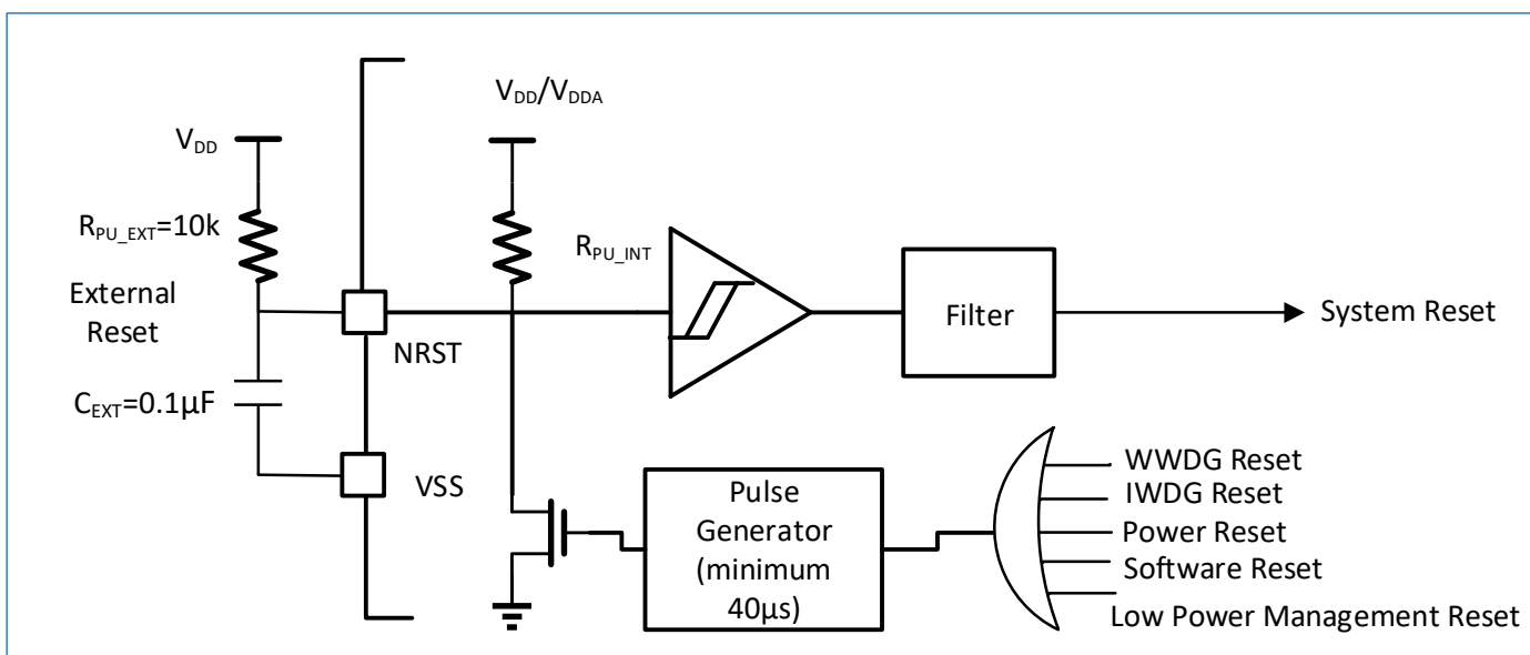
Figure 3-4 Reset Circuit
