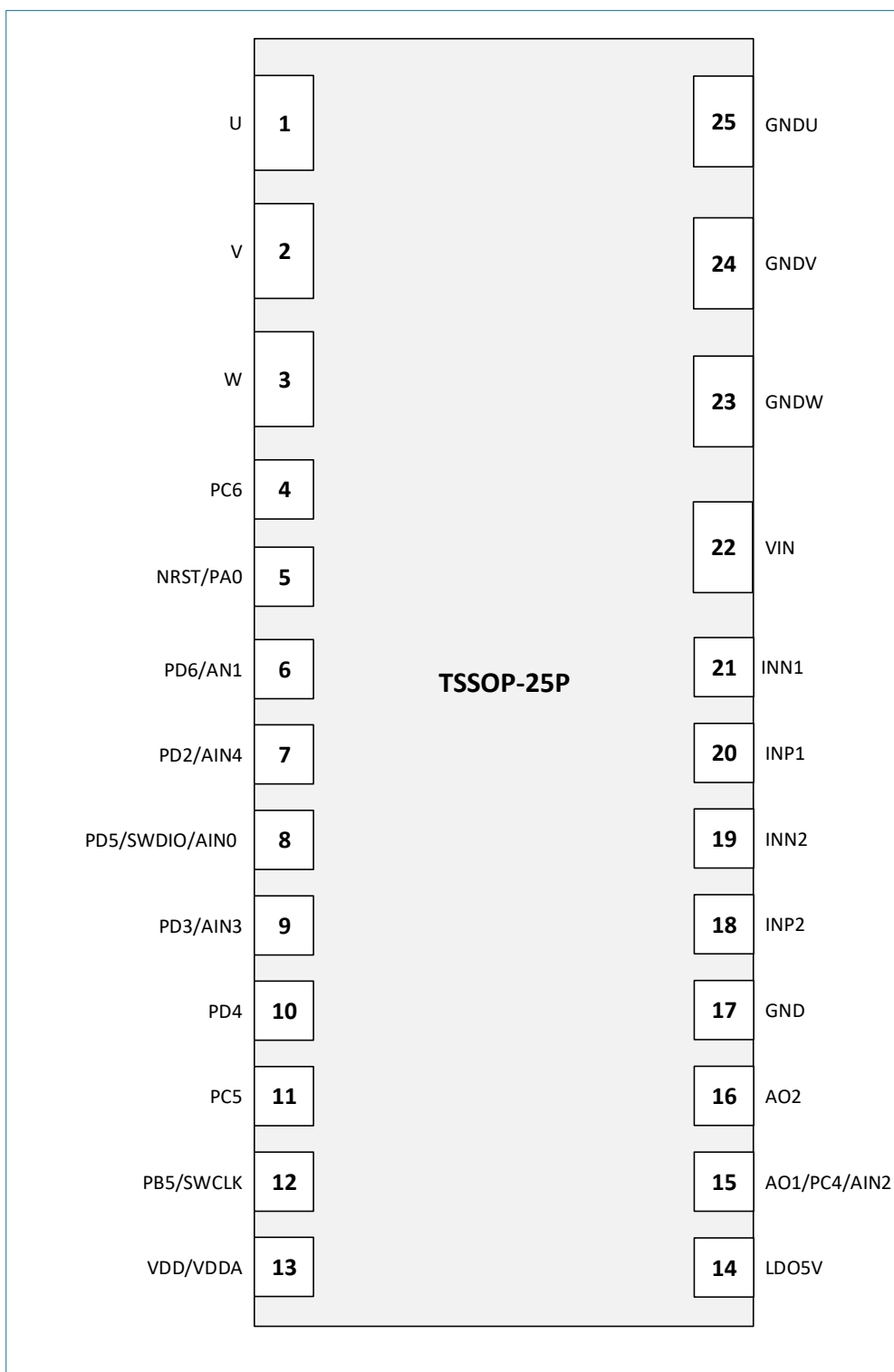
Figure 5-1 TSSOP-25P Package
