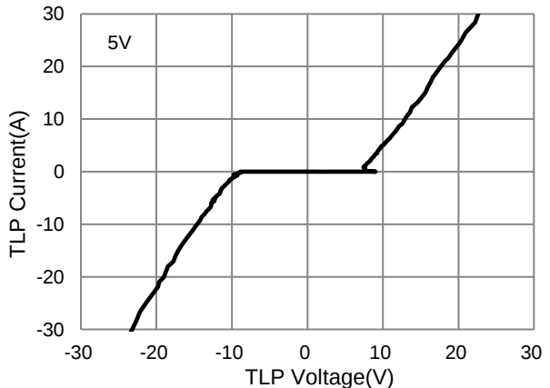
Fig.6 TLP Measurement
