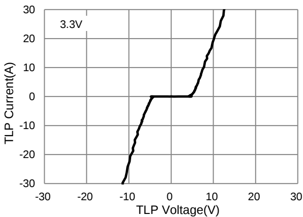
Fig.5 TLP Measurement
