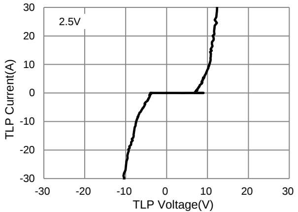
Fig.4 TLP Measurement
