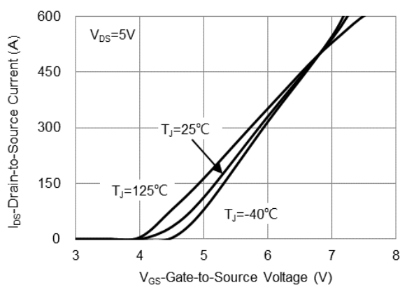
Fig.2 Transfer Characteristics
