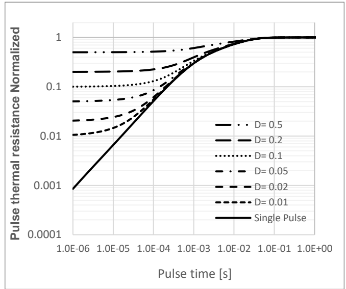
Fig.8 Max. Transient thermal impedance
