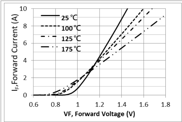
Fig.1 Forward Characteristics
