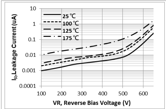
Fig.2 Reverse Characteristics
