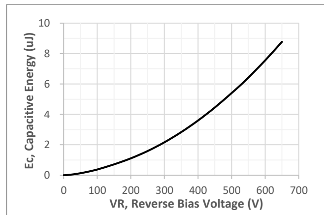
Fig.6 Capacitive Energy
