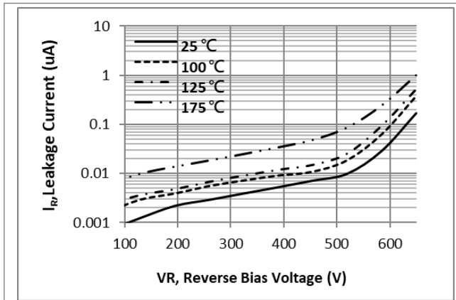
Fig.2 Reverse Characteristics
