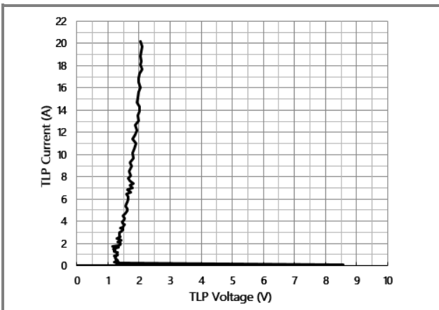
Fig.4 Positive TLP Measurement
