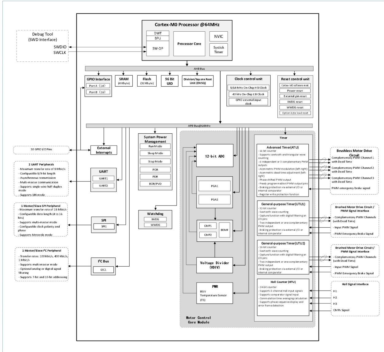
Figure 4-1 PM30225V-0401 Block Diagram
