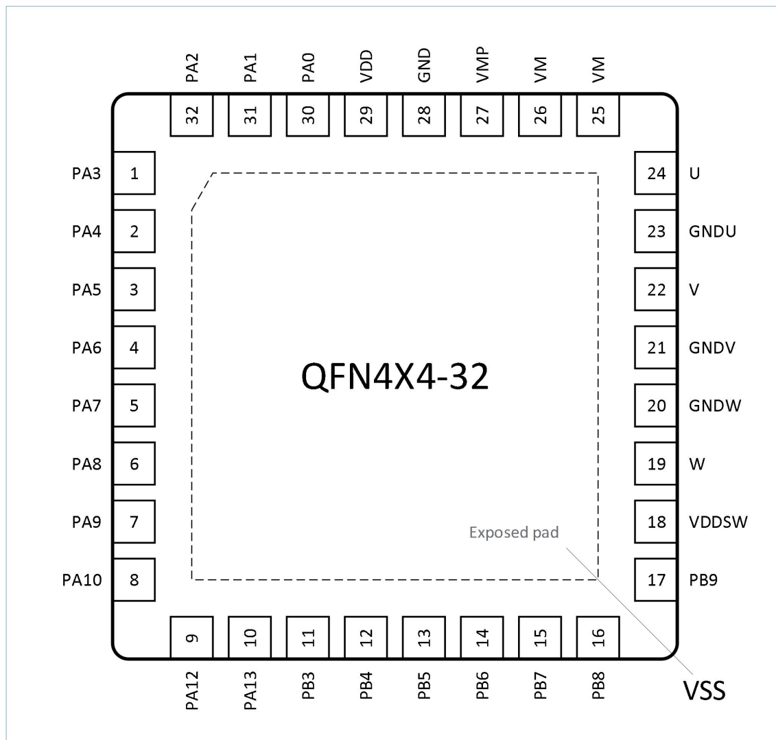
Figure 6-1 QFN4X4-32 Package
