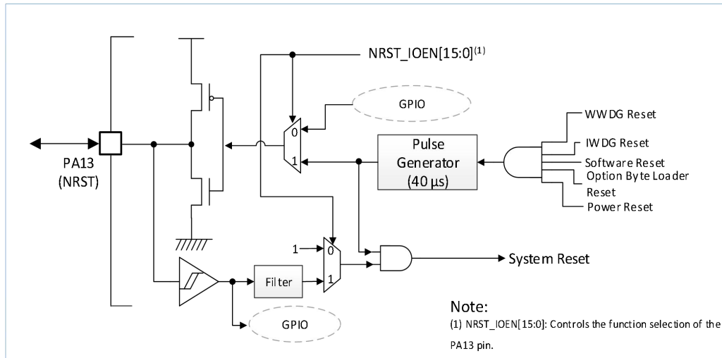
Figure 4-4 Reset Signals
