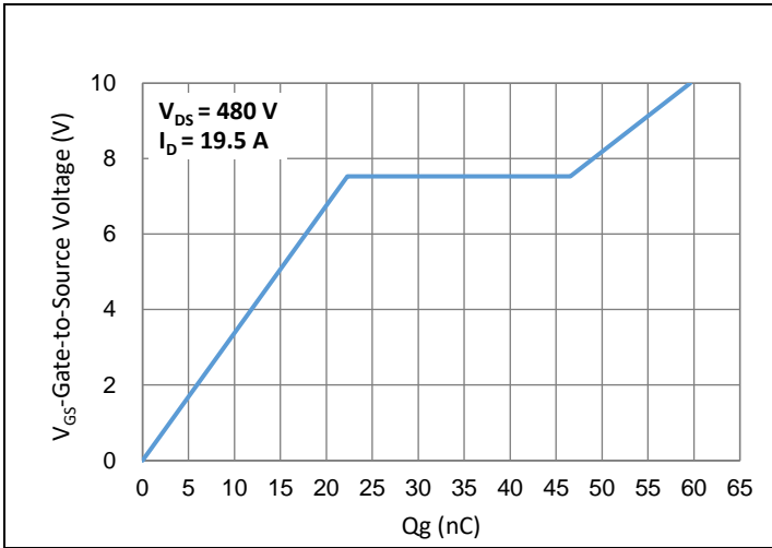
Fig.7 Gate-Charge Characteristics
